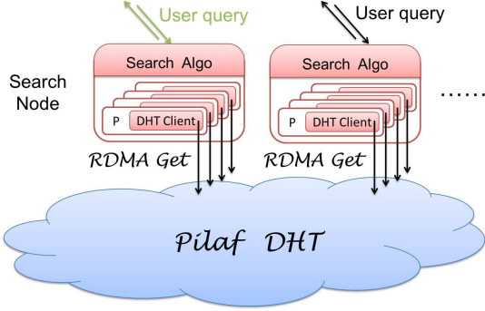
Figure 3: System Architecture
